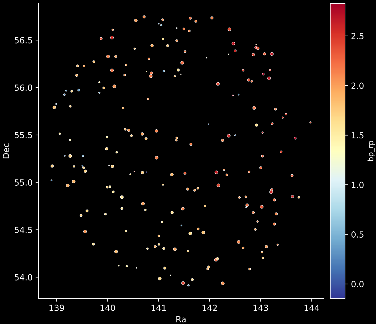
APOGEE DR17 Field: [139-04] Stars: 196
