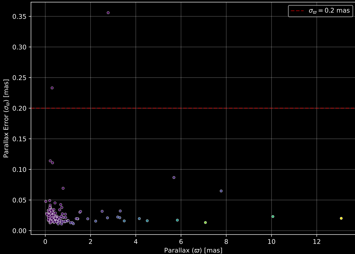
APOGEE DR17 Field: [139-04] Parallax Quality (n= 196)
